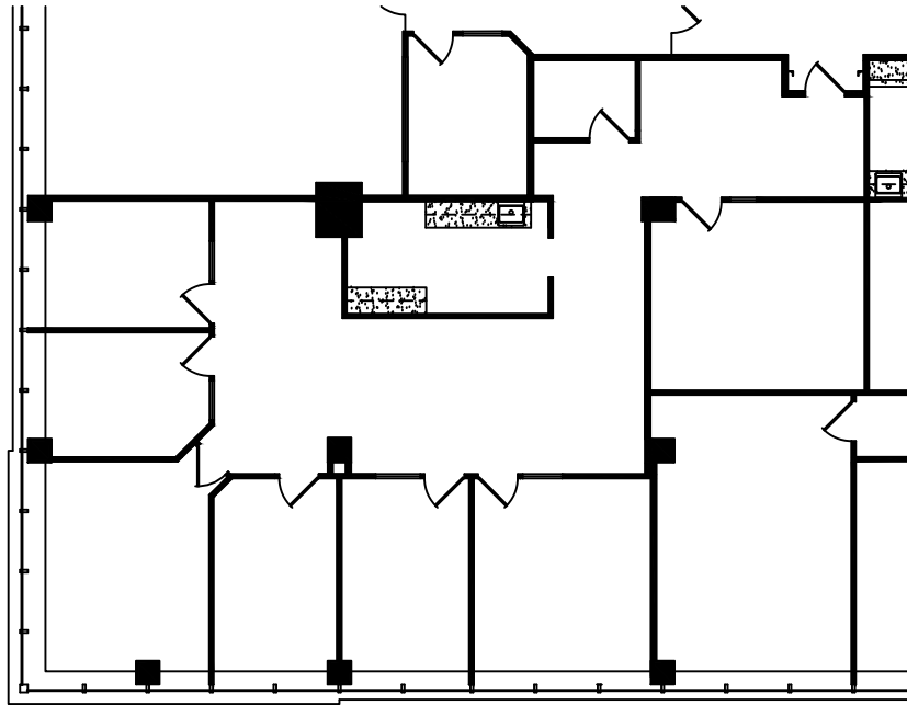
1 RECORD CONDITIONS SCALE: 1/16" = 1'0"
