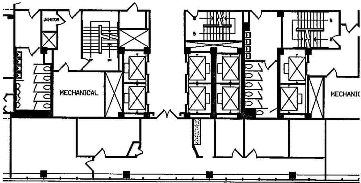
1 RECORD CONDITIONS SCALE: 1/16" = 1'-0"
