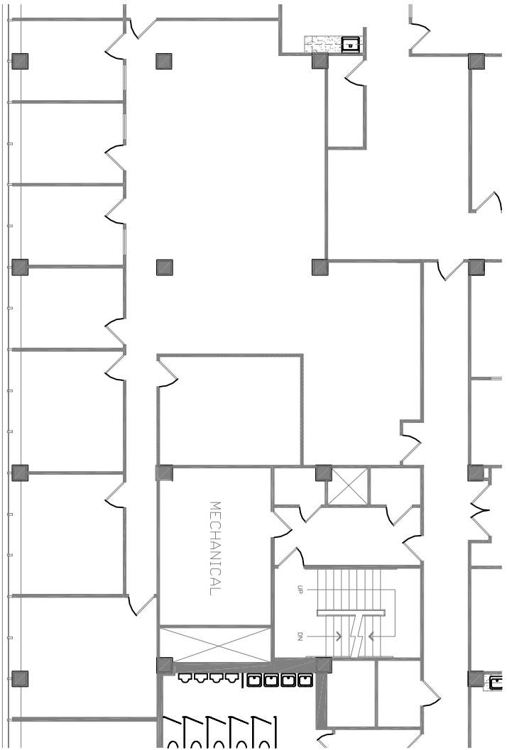
1 RECORD CONDITIONS SCALE: 1/16" = 1'-0"
